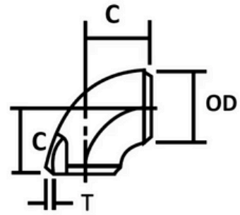
90° Elbow short radius
