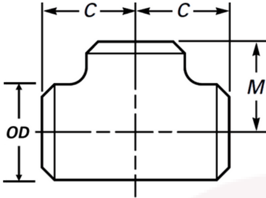
Equal Tee
