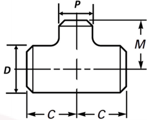
Unequal Tee
